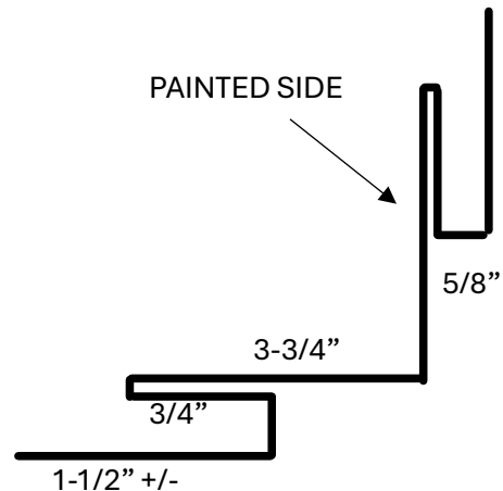
INSIDE CORNER 10'
