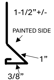
INSIDE CORNER 10'
