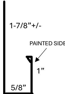
J CHANNEL 10'
